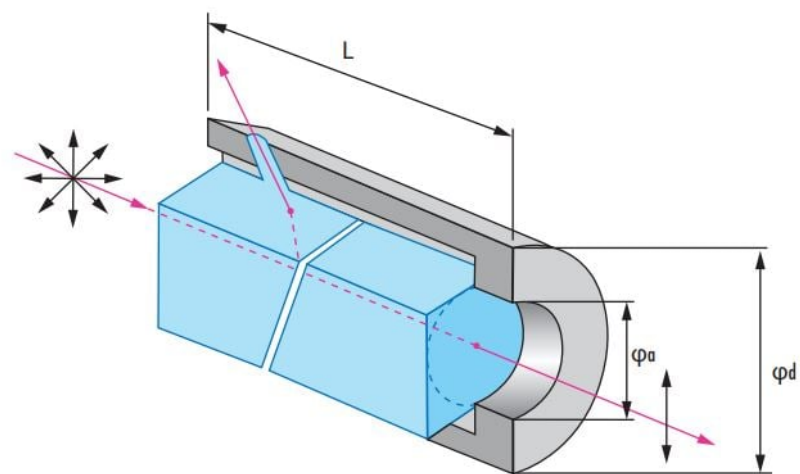
Glan-Laser Polarizers
