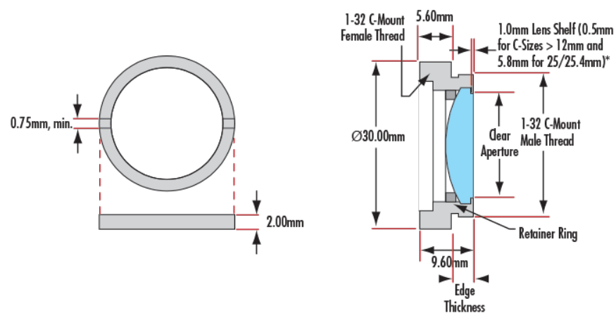
C-Thread Simple / Thin Lens Mount
