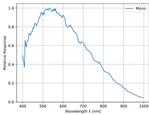
GMAX2509 Sensor QE Curve
