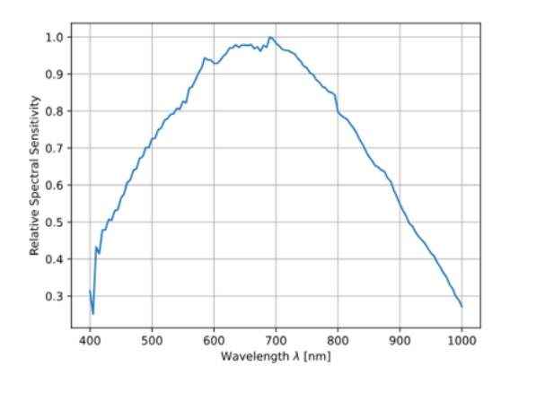
IMX900 Sensor QE Curve
