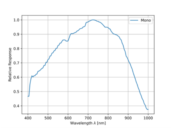
IMX676 Sensor QE Curve
