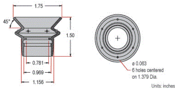
Style C) 0.95" Rubber Eyeguard
