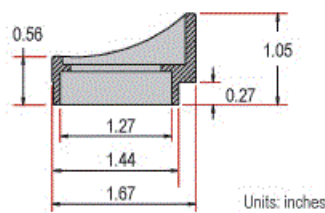
Style D) 35mm Super Rubber Eyeguard
