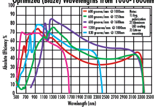
Typical Efficiency Curves for Ruled Gratings Optimized (Blaze) Wavelengths from 1000-1600nm
