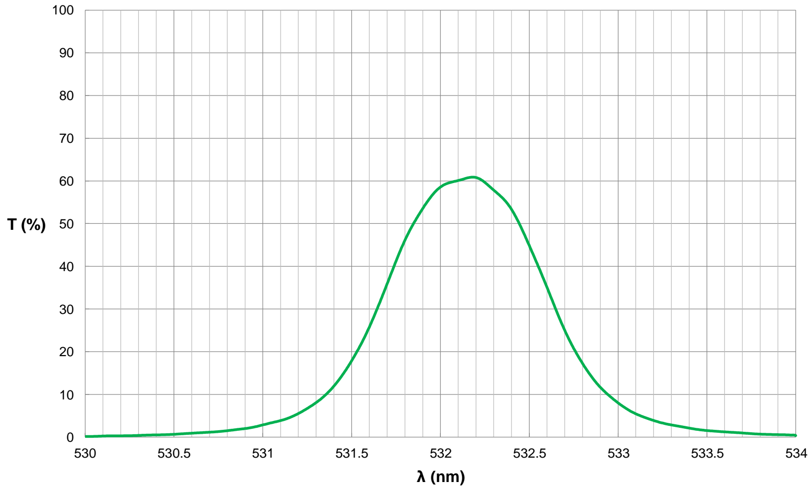
Ultra Narrow Traditional Coated Bandpass Filter, 532nm, 1.00 FWHM FOR REFERENCE ONLY
