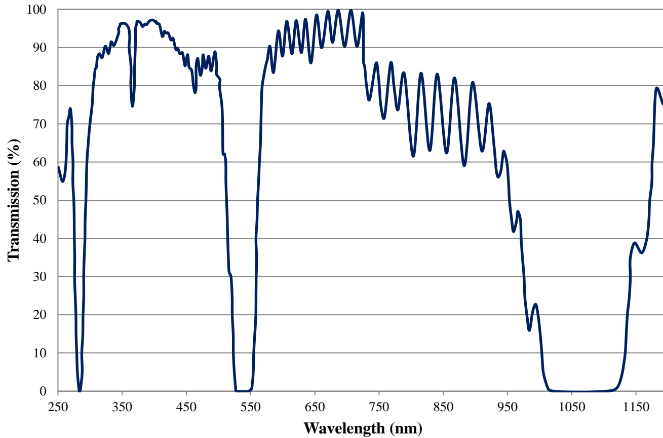
355nm T, 532 & 1064nm R Harmonic Separator Typical Transmission FOR REFERENCE ONLY
