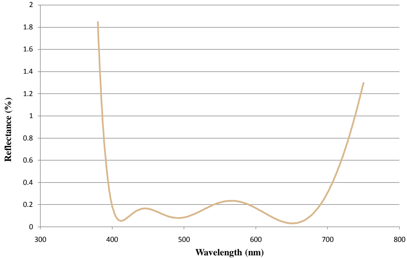
VIS 0° [425-675nm] Anti-Reflection Coating Performance FOR REFERENCE ONLY
